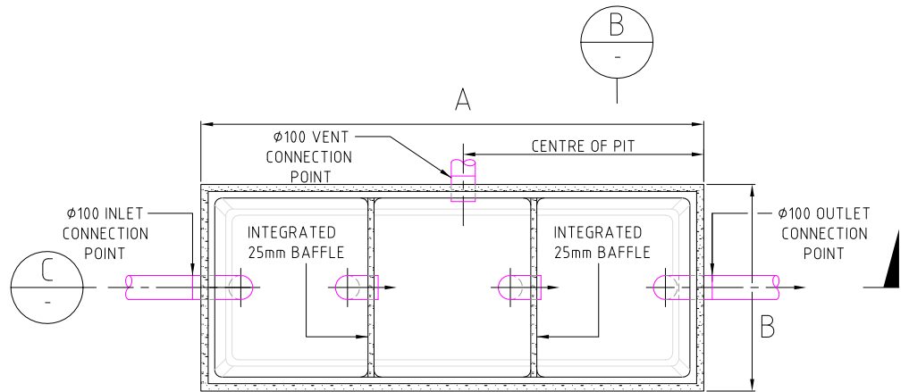
A OPEN TANK PLAN VIEW - NOT TO SCALE
