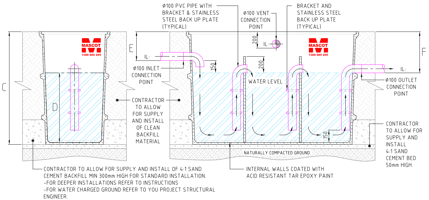
B END SECTION - NOT TO SCALE
